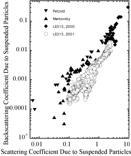
Fig. 3. Backscattering coefficient due to suspended particles (SP) versus scattering coefficient due to SP.
