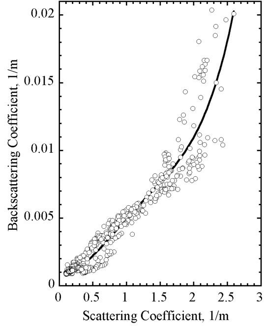
Fig. 6. Backscattering coefficient as a function of scattering coefficient for the LEO-15 (2001) PHFs.
