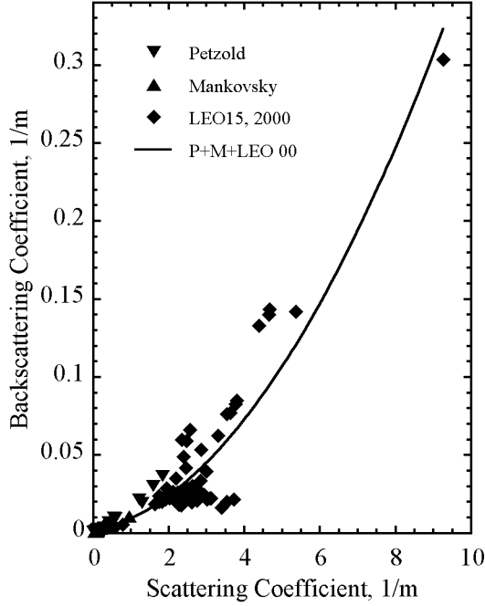
Fig. 5. The same as Fig. 2 only with the addition of LEO-15 (2000) PHFs measured near New Jersey coast.
